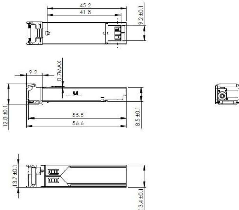
Mechanical Drawing
